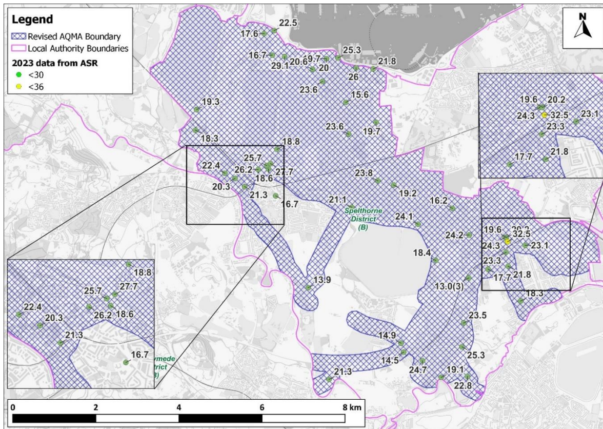
Figure 1 Spelthorne AQMA showing 2023 annual mean monitored NO 2 concentrations, all below the air quality objective
